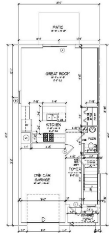
SCHEME 1 FIRST FLOOR PLAN
